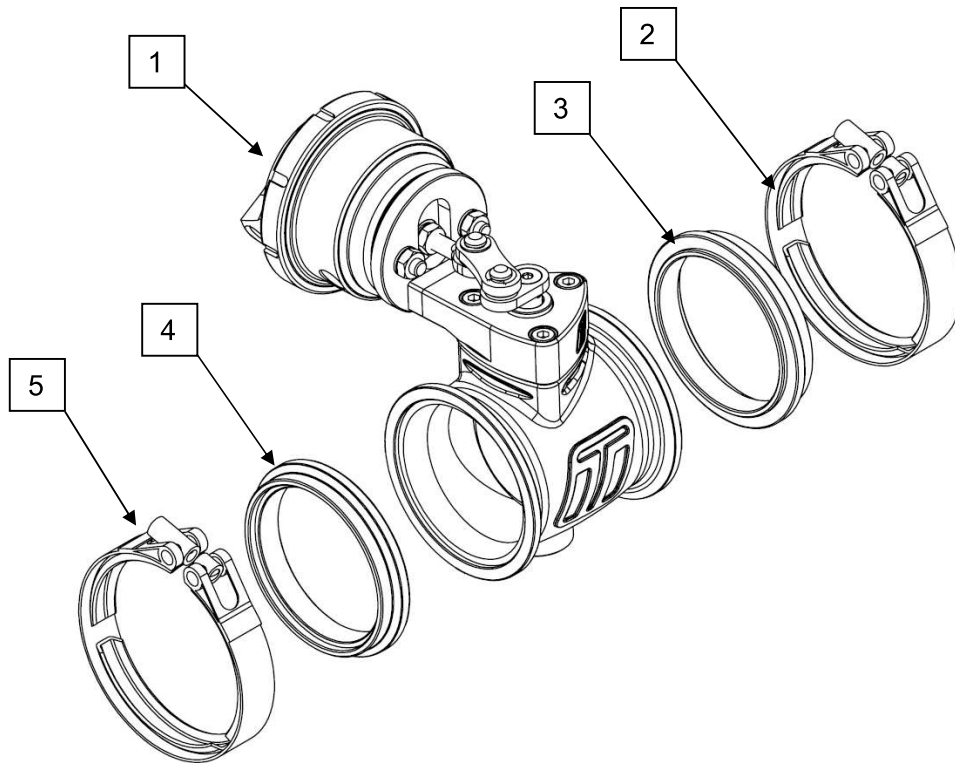
Figure 1 - Kit Contents
