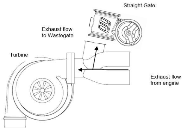
Figure 7 - Not Recommended - Less than 90 Degree Mounting. An angle mounting as shown in not recommended and gives extremely poor exhaust flow to the Straight Gate which can contribute to poor boost control and over boosting.
