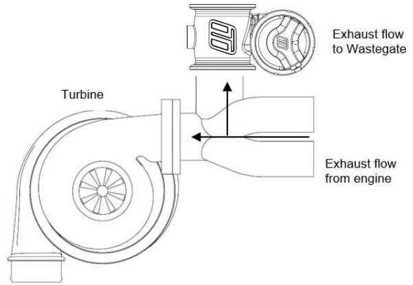
Figure 6 - 90 Degree mounting 90 Degree mounting of the Straight Gate and in some circumstances may contribute to over boosting.
