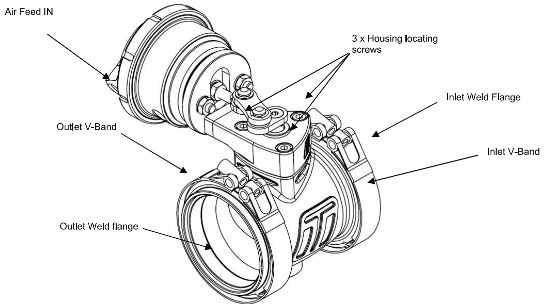
Figure 1 - Pneumatic Straight Gate Overview
