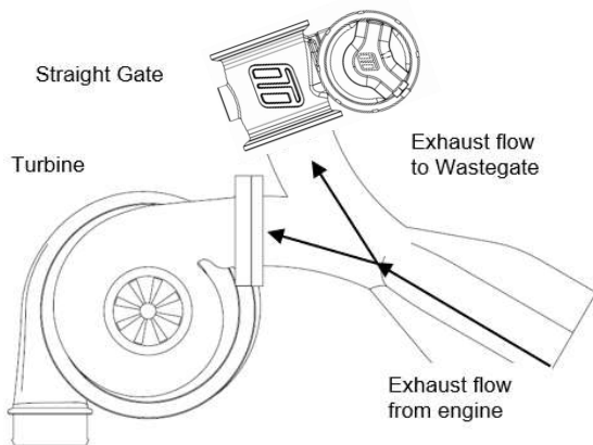
Figure 4 - Best flow - Symmetric mounting Symmetric mounting allows an excellent flow of exhaust to the Straight Gate.
