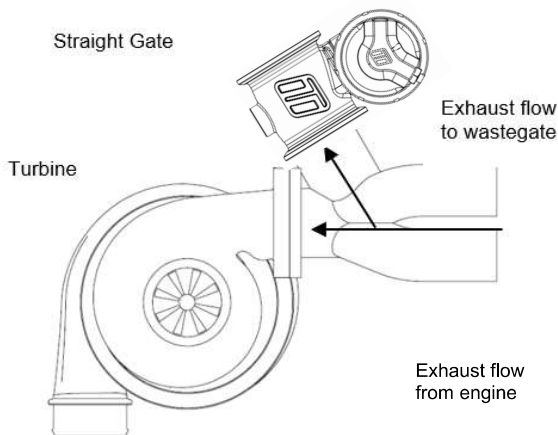
Figure 5 - Good Flow - Angle mounting Angle mounting allows a good flow of exhaust flow to the Straight Gate.
